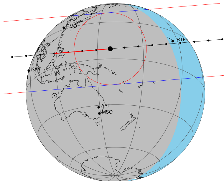
2047-05-11T16:12:32.7500 α: 18 14 26.6617 δ: -22 19 02.764 C/A 0.468" PA 355.18 deg v_sky -16.68 km/s D 09.28 AU Credit: Styled after SORA/Lucky Star
