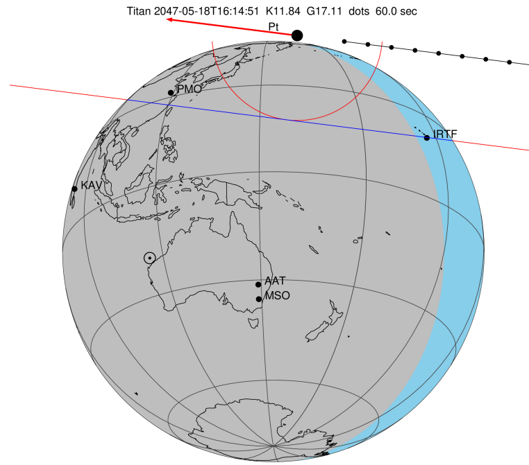
2047-05-18T16:14:51.1600 α: 18 12 40.5235 δ: -22 17 28.634 C/A 0.985" PA 7.18 deg v_sky -11.97 km/s D 09.21 AU
