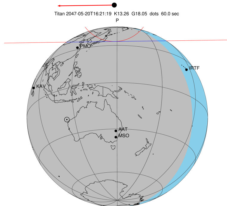
2047-05-20T16:21:19.0500 α: 18 12 20.6201 δ: -22 17 09.557 C/A 1.184" PA 359.21 deg v_sky - 9.82 km/s D 09.20 AU Credit: Styled after SORA/Lucky Star
