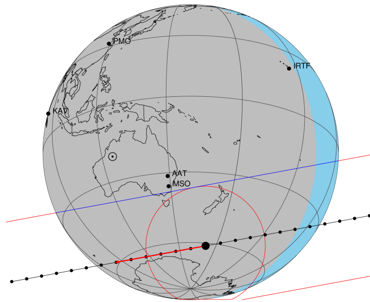
2047-05-22T15:35:39.6700 cc: 18 12 02.2456 d: -22 17 35.382 C/A 0.615" PA 169.55 deg v_sky -10.89 km/s D 09.18 AU Credit: Styled after SORA/Lucky Star
