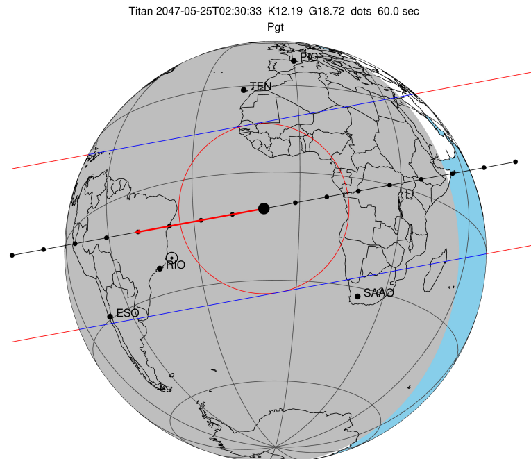
2047-05-25T02:30:33.6900 cc: 18 11 32.3208 s: -22 19 00.751 C/A 0.204" PA 349.45 deg v_sky -16.13 km/s D 09.15 AU Credit: Styled after SORA/Lucky Star
