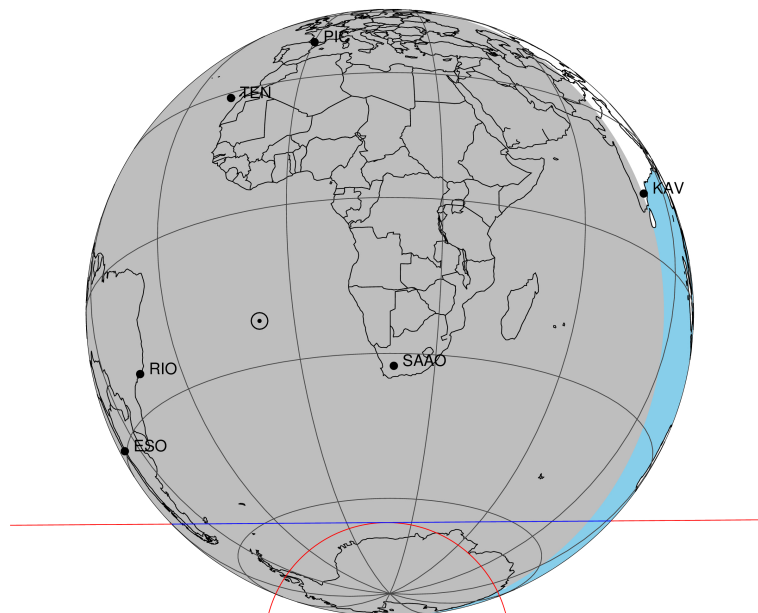
2047-05-29T00:27:30.2000 cc: 18 10 18.2472 s -22 20 33.9611 s C/A 1.056" PA 179.59 deg v_sky -22.83 km/s D 09.11 AU Credit: Styled after SORA/Lucky Star
