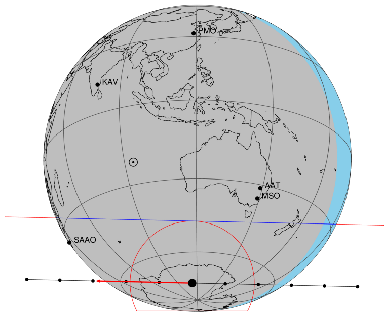
2047-05-29T17:41:56.8400 cc: 18 10 02.7625 s: -22 20 32.597 C/A 0.786" PA 181.26 deg v_sky -22.85 km/s D 09.11 AU Credit: Styled after SORA/Lucky Star
