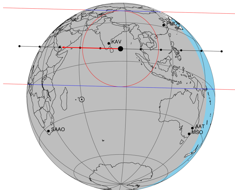
2047-05-29T19:58:10.9900 α: 18 10 00.7240 δ: -22 20 33.204 C/A 0.494" PA 1.47 deg v_sky -22.83 km/s D 09.11 AU Credit: Styled after SORA/Lucky Star
