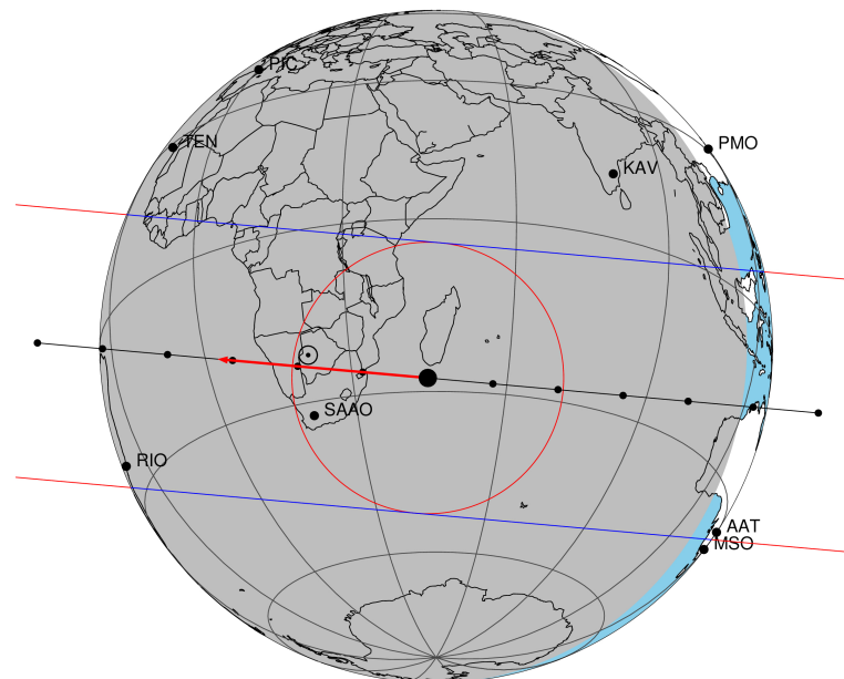
2047-05-31T22:29:51.2600 cc: 18 09 17.2066 s: -22 19 56.295 C/A 0.092" PA 185.18 deg v_sky -20.64 km/s D 09.10 AU Credit: Styled after SORA/Lucky Star
