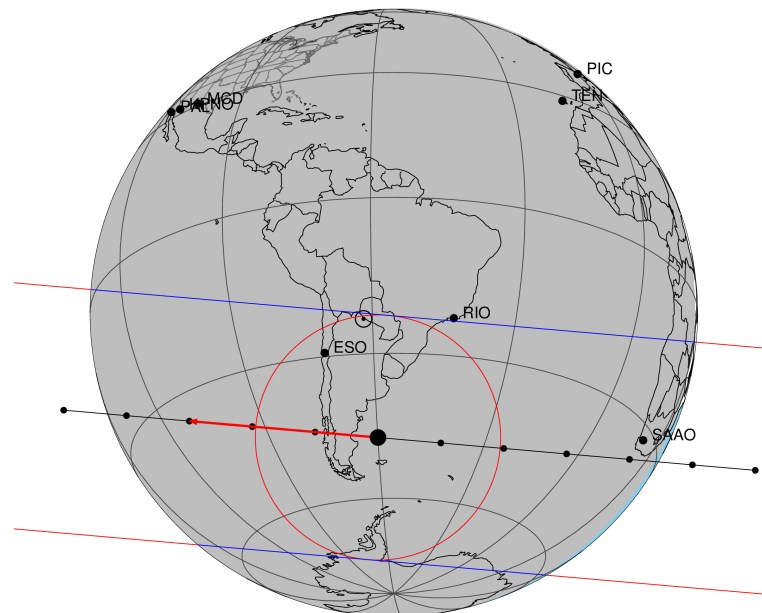
2047-06-17T04:08:08.2700 cc: 18 04 21.5963 s: -22 21 24.641 C/A 0.403" PA 184.99 deg v_sky -22.09 km/s D 09.03 AU Credit: Styled after SORA/Lucky Star
