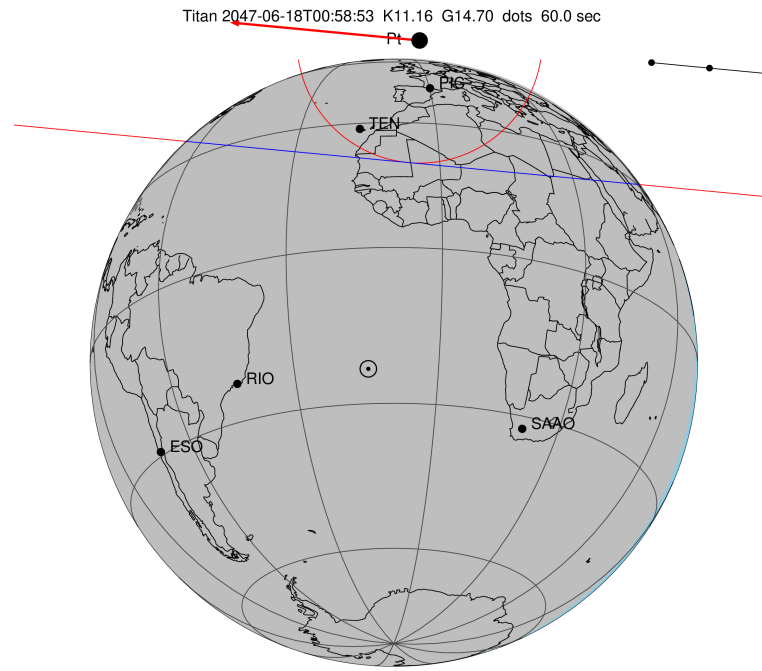
2047-06-18T00:58:53.3800 α: 18 04 04.1180 δ: -22 21 03.779 C/A 1.037" PA 5.45 deg v_sky -20.38 km/s D 09.03 AU Credit: Styled after SORA/Lucky Star
