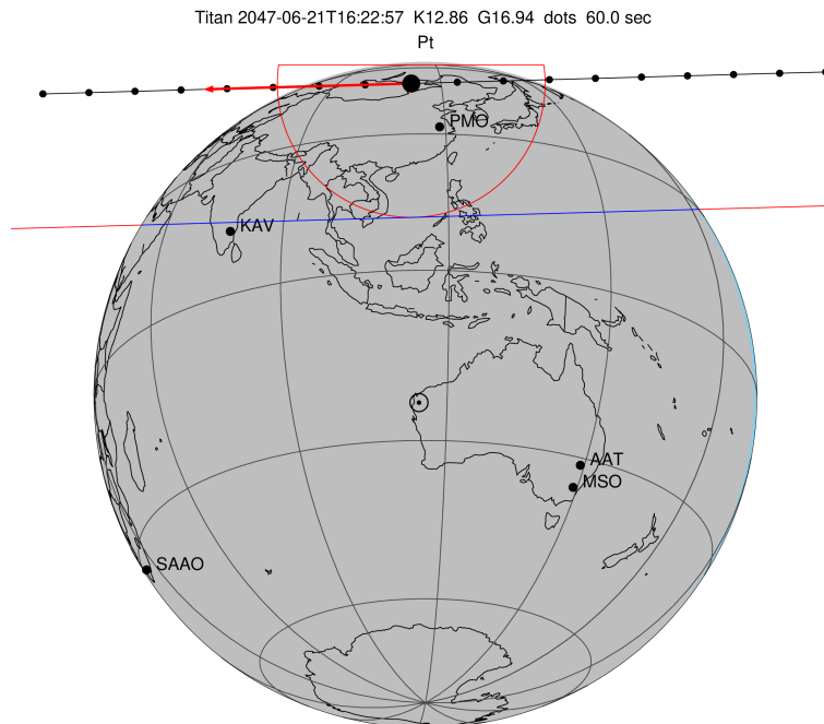
2047-06-21T16:22:57.600000 cc: 18 03 05.1250 d: -22 20 14.488 C/A 0.919" PA 358.40 deg v_sky -14.77 km/s D 09.04 AU Credit: Styled after SORA/Lucky Star
