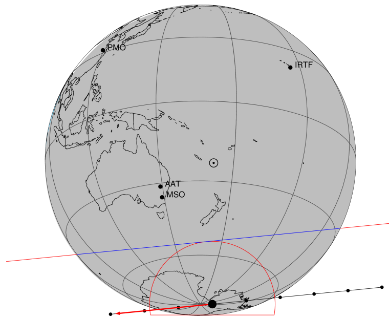
2047-06-27T12:35:22.8400 cc: 18 01 27.0310 & -22 23 08.860 C/A 0.905" PA 174.32 deg v_sky -23.31 km/s D 09.03 AU Credit: Styled after SORA/Lucky Star
