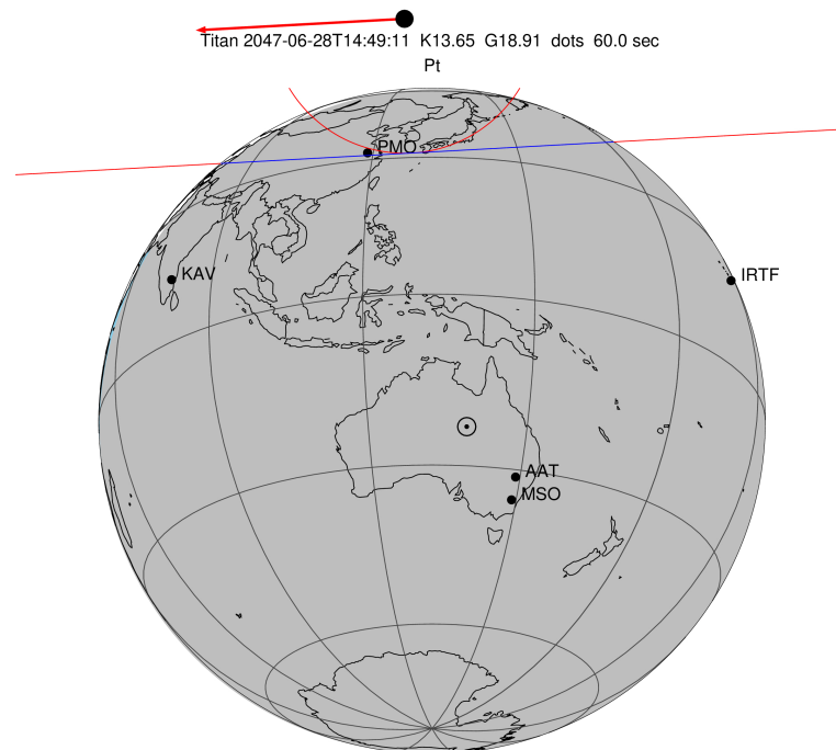
2047-06-28T14:49:11.9200 cc: 18 01 02.00666 s: -22 23 37.718 C/A 1.179" PA 356.85 deg v_sky -24.86 km/s D 09.03 AU Credit: Styled after SORA/Lucky Star
