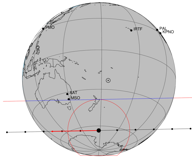
2047-06-29T11:41:41.9700 cc: 18 00 41.1666 d: -22 23 46.641 C/A 0.652" PA 178.86 deg v_sky -25.43 km/s D 09.03 AU Credit: Styled after SORA/Lucky Star
