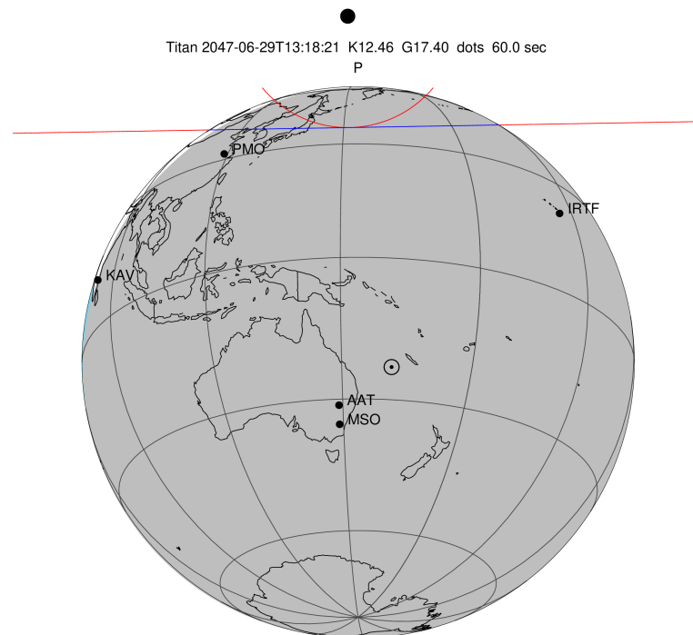
2047-06-29T13:18:21.0600 cc: 18 00 39.5449 d: -22 23 48.930 C/A 1.223" PA 359.02 deg v_sky -25.45 km/s D 09.03 AU Credit: Styled after SORA/Lucky Star
