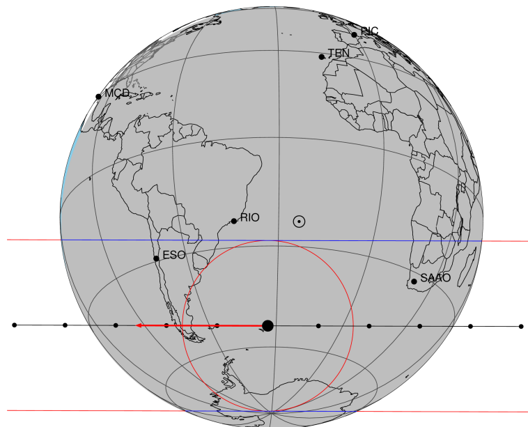
2047-06-30T01:39:22.4000 α: 18 00 27.0747 δ: -22 23 48.434 C/A 0.497" PA 180.16 deg v_sky -25.46 km/s D 09.03 AU
