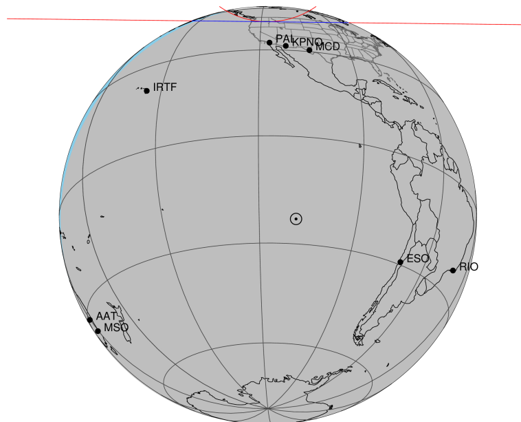
2047-06-30T07:19:27.1800 α: 18 00 21.3618 δ: -22 23 49.653 C/A 1.296" PA 0.67 deg v_sky -25.39 km/s D 09.03 AU Credit: Styled after SORA/Lucky Star
