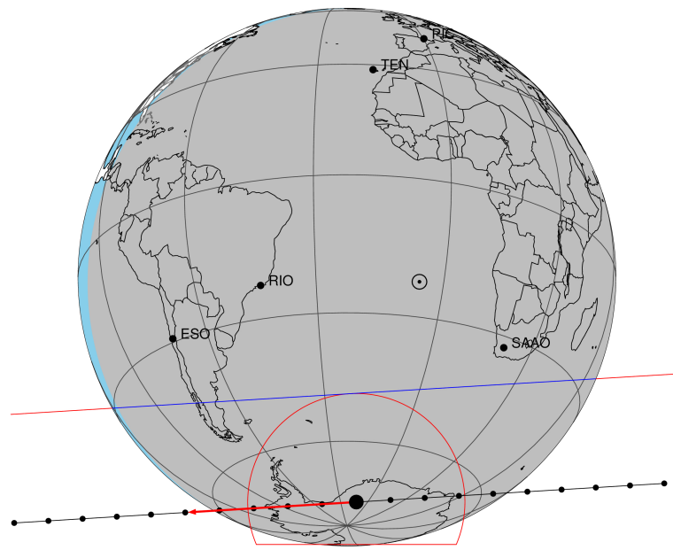
2047-07-08T00:28:29.5300 cc: 17 57 59.7067 & -22 21 50.588 C/A 0.812" PA 176.52 deg v_sky -13.55 km/s D 09.07 AU Credit: Styled after SORA/Lucky Star
