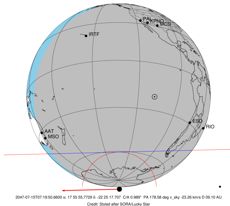
Titan 2047-07-15T07:19:50 K10.36 G17.30 dots 60.0 sec P
