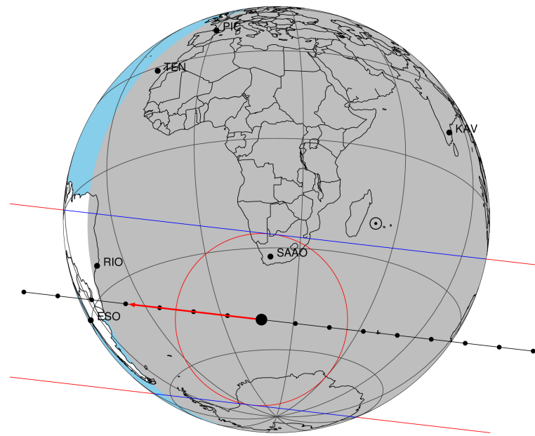
2047-07-19T20:35:58.0100 cc: 17 54 25.2505 s: -22 24 09.432 C/A 0.456" PA 186.63 deg v_sky -17.04 km/s D 09.13 AU Credit: Styled after SORA/Lucky Star
