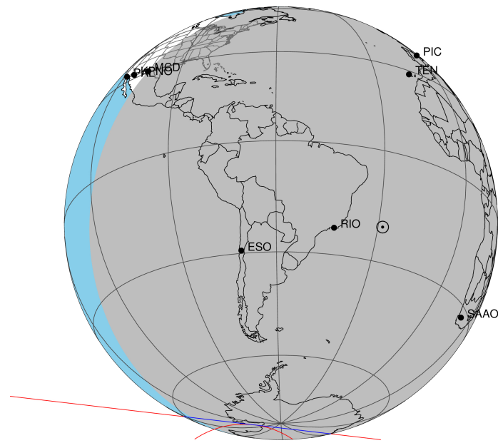
2047-07-20T02:00:31.8700 cc: 17 54 21.7264 & -22 24 02.881 C/A 1.293" PA 186.69 deg v_sky -16.51 km/s D 09.14 AU Credit: Styled after SORA/Lucky Star
