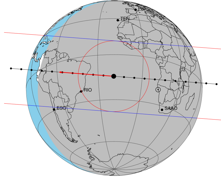
2047-07-21T23:14:44.9600 α: 17 53 56.3743 δ: -22 23 26.839 C/A 0.128" PA 4.42 deg v_sky -12.44 km/s D 09.16 AU Credit: Styled after SORA/Lucky Star
