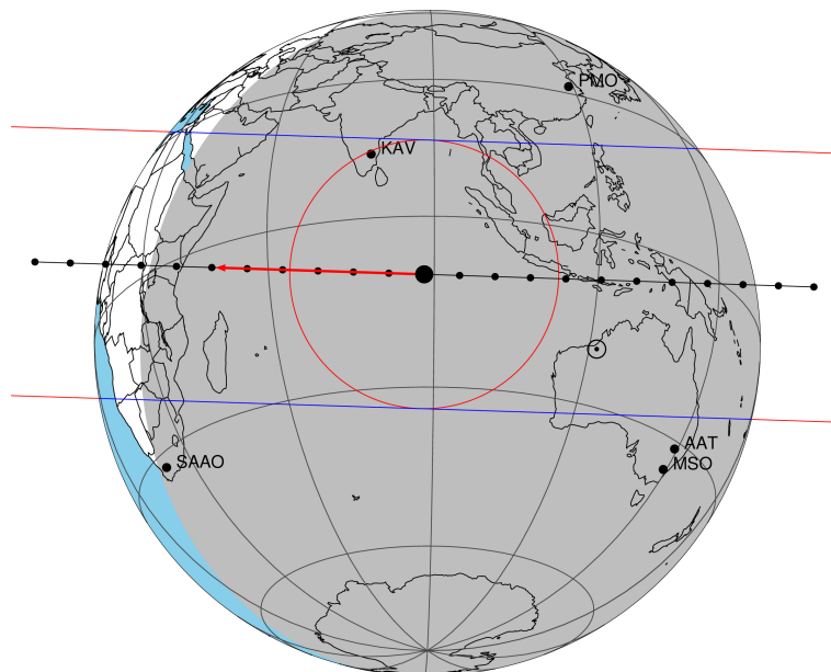
2047-07-22T16:00:05.5100 α: 17 53 48.6325 δ: -22 23 20.867 C/A 0.197" PA 1.86 deg v_sky -11.31 km/s D 09.16 AU Credit: Styled after SORA/Lucky Star
