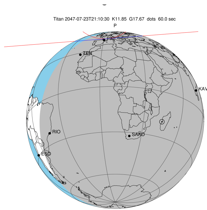
2047-07-23T21:10:30.2800 cc: 17 53 36.5073 s: -22 23 25.296 C/A 1.272" PA 355.49 deg v_sky -10.23 km/s D 09.18 AU Credit: Styled after SORA/Lucky Star
