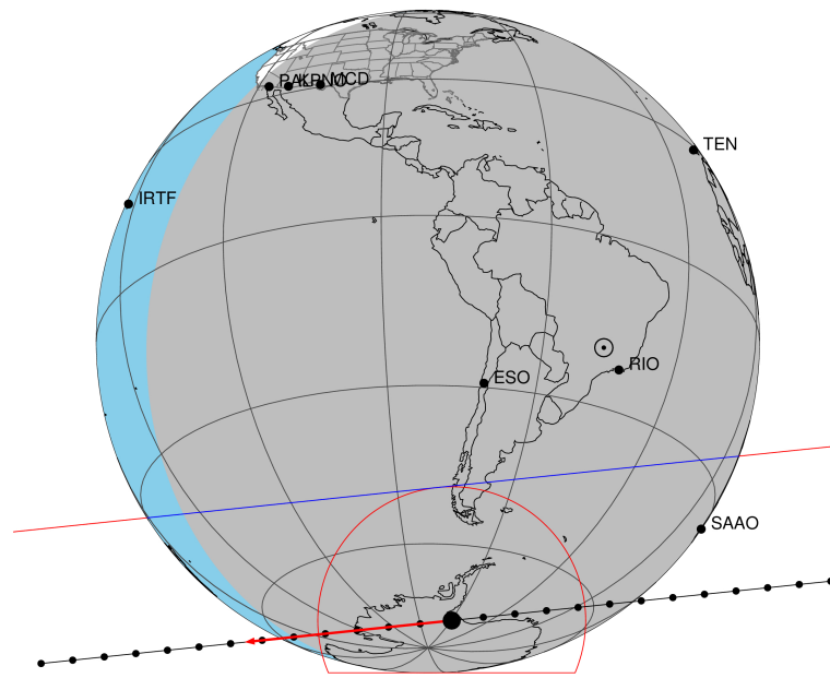
2047-07-24T03:16:48.6500 cc: 17 53 34.0757 & -22 23 26.297 C/A 0.809" PA 174.04 deg v_sky -10.18 km/s D 09.18 AU Credit: Styled after SORA/Lucky Star
