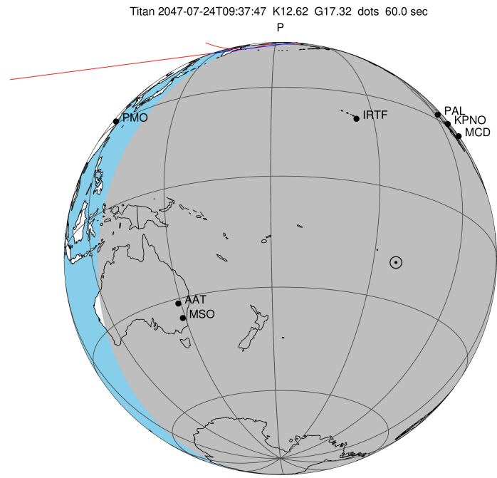
2047-07-24T09:37:47.0000 cc: 17 53 31.5923 s -22 23 32.482 C/A 1.327" PA 352.60 deg v_sky -10.18 km/s D 09.18 AU Credit: Styled after SORA/Lucky Star
