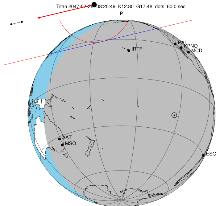
2047-07-26T08:20:49.3700 cc: 17 53 12.2012 d: -22 24 25.995 C/A 1.146" PA 346.62 deg v_sky -12.04 km/s D 09.20 AU Credit: Styled after SORA/Lucky Star
