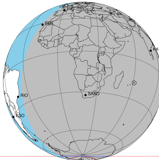
2047-07-31T20:02:32.7000 cc: 17 51 48.7427 & -22 26 54.430 C/A 1.282" PA 179.96 deg v_sky -18.84 km/s D 09.24 AU Credit: Styled after SORA/Lucky Star
