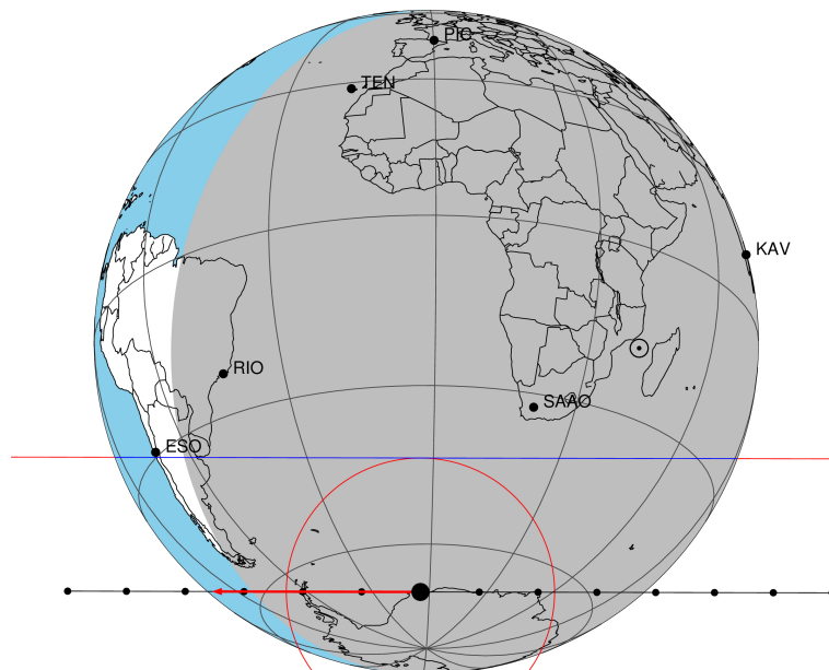
2047-07-31T21:23:33.5100 cc: 17 51 47.7575 & -22 26 54.983 C/A 0.717" PA 180.13 deg v_sky -18.82 km/s D 09.24 AU Credit: Styled after SORA/Lucky Star
