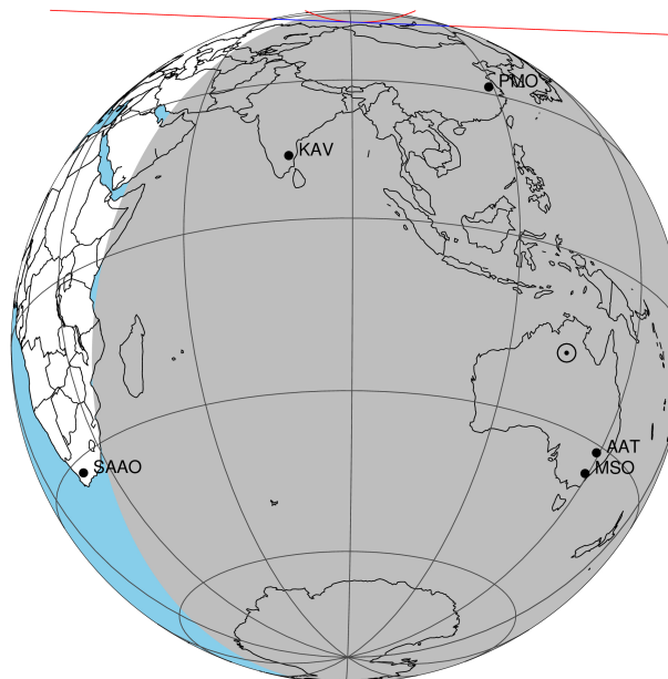
2047-08-01T15:17:03.5200 α: 17 51 34.8938 δ: -22 26 53.283 C/A 1.301" PA 2.25 deg v_sky -18.23 km/s D 09.25 AU Credit: Styled after SORA/Lucky Star
