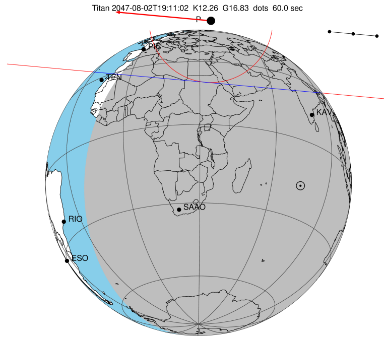
2047-08-02T19:11:02.9700 α: 17 51 16.0964 δ: -22 26 35.827 C/A 1.009" PA 5.27 deg v_sky -16.53 km/s D 09.26 AU Credit: Styled after SORA/Lucky Star
