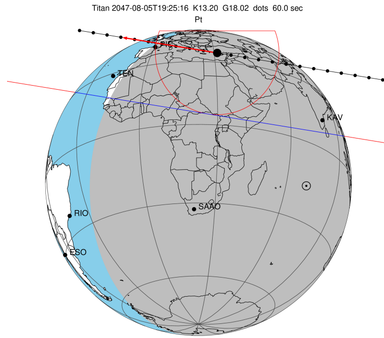
2047-08-05T19:25:16.9200 α: 17 50 39.5304 δ: -22 25 26.150 C/A 0.811" PA 9.26 deg v_sky - 9.70 km/s D 09.30 AU Credit: Styled after SORA/Lucky Star
