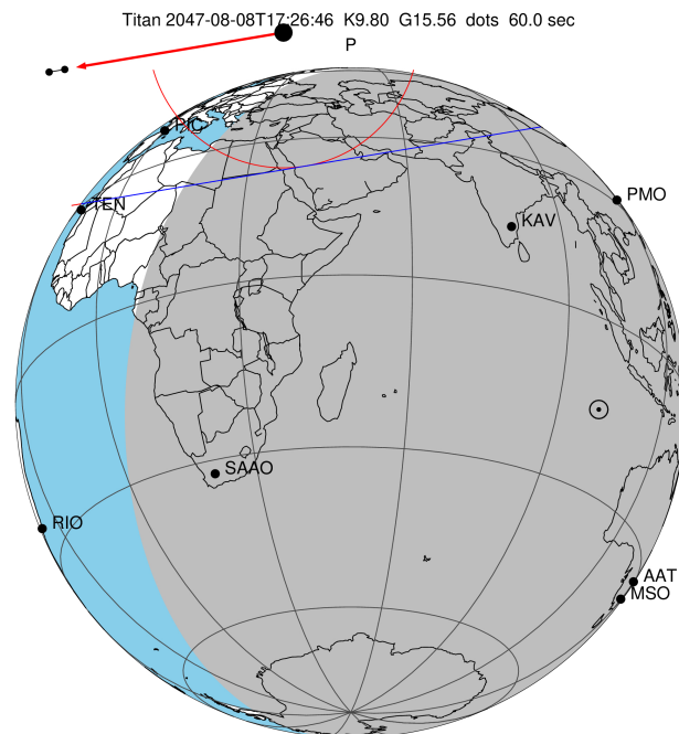
2047-08-08T17:26:46.5700 α: 17 50 21.1713 δ: -22 25 08.093 C/A 1.057" PA 350.48 deg v_sky - 5.02 km/s D 09.34 AU Credit: Styled after SORA/Lucky Star
