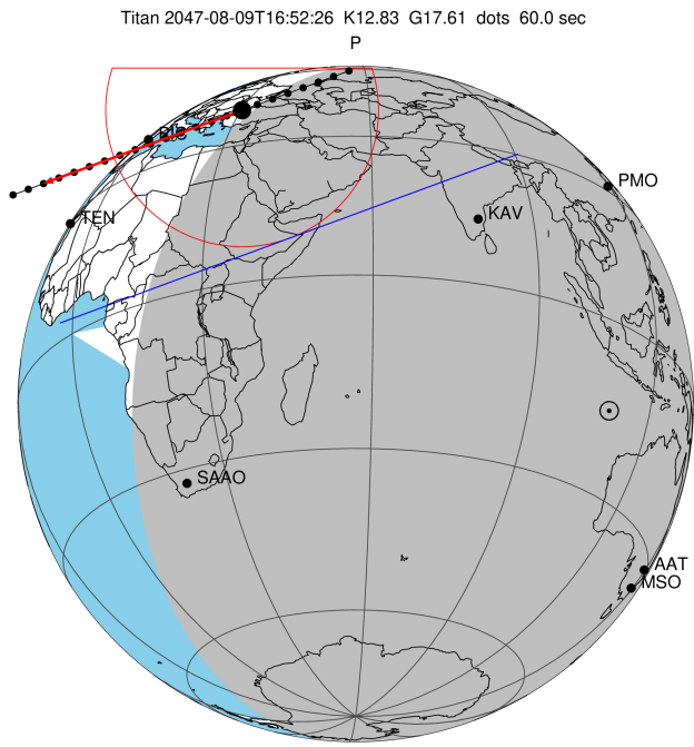
2047-08-09T16:52:26.5300 α: 17 50 16.8659 δ: -22 25 24.137 C/A 0.876" PA 339.76 deg v_sky - 5.12 km/s D 09.35 AU Credit: Styled after SORA/Lucky Star
