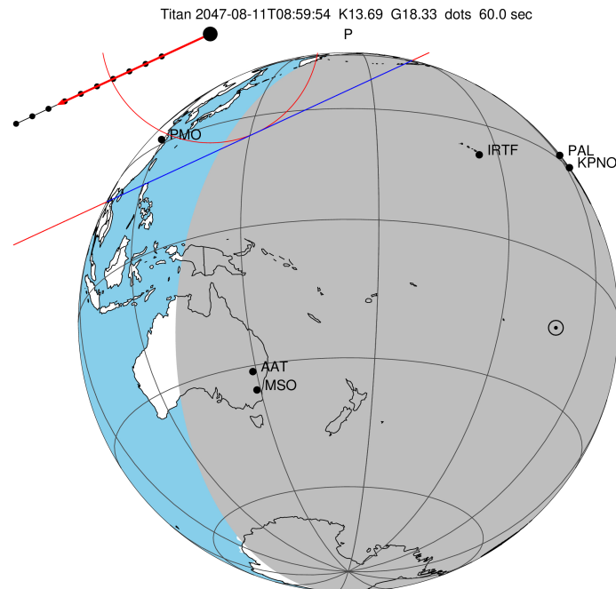
2047-08-11T08:59:54.5700 α: 17 50 08.5830 δ: -22 26 15.925 C/A 1.112" PA 335.14 deg v_sky - 7.01 km/s D 09.37 AU Credit: Styled after SORA/Lucky Star
