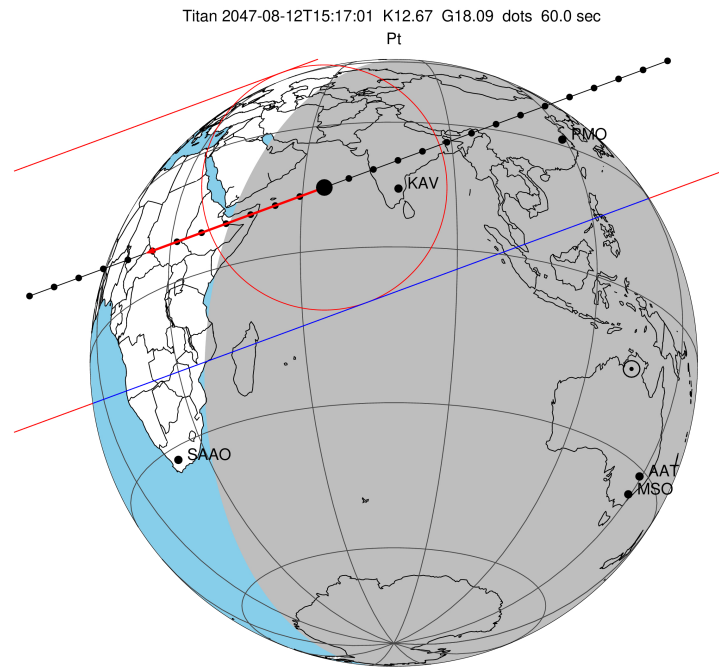
2047-08-12T15:17:01.1200 α: 17 49 59.9713 δ: -22 27 05.379 C/A 0.582" PA 339.75 deg v_sky - 9.15 km/s D 09.39 AU Credit: Styled after SORA/Lucky Star
