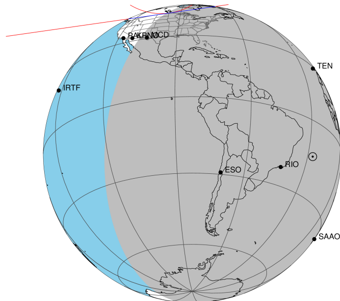
2047-08-15T01:52:01.8300 cc: 17 49 35.9990 & -22 28 28.019 C/A 1.270" PA 351.85 deg v_sky -12.60 km/s D 09.41 AU
