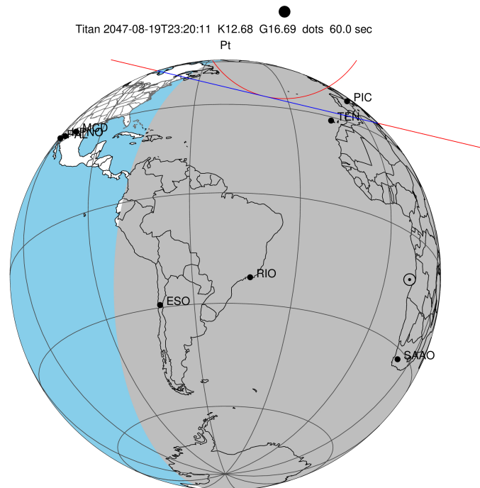
2047-08-19T23:20:11.7200 α: 17 48 45.1552 δ: -22 28 05.901 C/A 1.163" PA 13.37 deg v_sky - 7.67 km/s D 09.48 AU Credit: Styled after SORA/Lucky Star
