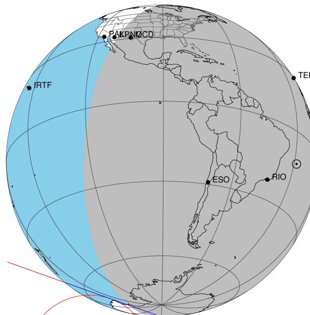
2047-08-21T01:56:30.9400 α: 17 48 39.0967 δ: -22 27 39.157 C/A 1.247" PA 199.55 deg v_sky - 4.99 km/s D 09.50 AU
