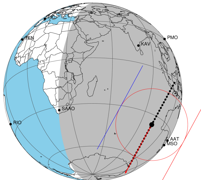
2047-08-28T16:15:04.5200 α: 17 48 39.1565 δ: -22 29 22.620 C/A 0.691" PA 118.56 deg v_sky - 3.78 km/s D 09.61 AU Credit: Styled after SORA/Lucky Star
