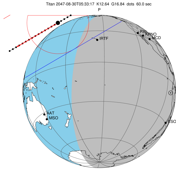
2047-08-30T05:33:17.3700 α: 17 48 34.8035 δ: -22 30 22.368 C/A 0.956" PA 329.62 deg v_sky - 5.16 km/s D 09.63 AU Credit: Styled after SORA/Lucky Star
