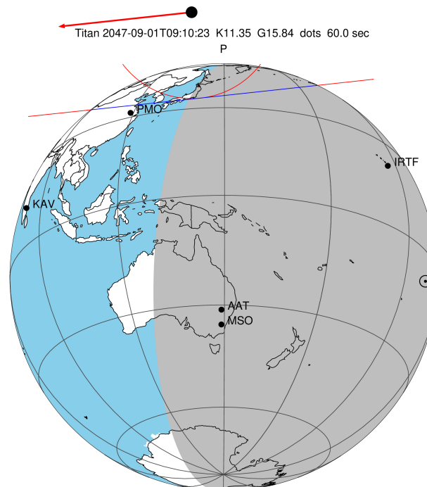
2047-09-01T09:10:23.6400 α: 17 48 24.4231 δ: -22 31 06.791 C/A 1.137" PA 353.84 deg v_sky - 5.76 km/s D 09.66 AU Credit: Styled after SORA/Lucky Star
