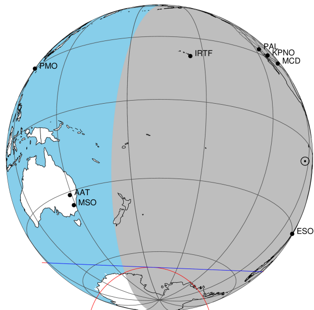
2047-09-02T06:17:08.0200 α: 17 48 20.1339 δ: -22 31 06.7731 C/A 1.014" PA 182.35 deg v_sky - 5.12 km/s D 09.68 AU Credit: Styled after SORA/Lucky Star
