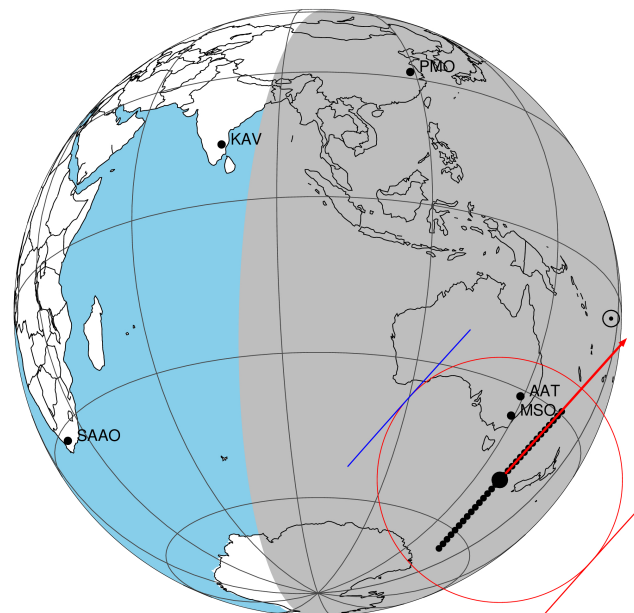
2047-09-05T12:21:44.5900 α: 17 48 13.6002 δ: -22 30 20.212 C/A 0.735" PA 131.87 deg v_sky + 2.15 km/s D 09.74 AU Credit: Styled after SORA/Lucky Star
