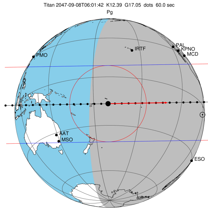
2047-09-08T06:01:42.5700 cc: 17 48 25.0551 d: -22 29 45.940 C/A 0.089" PA 359.02 deg v_sky + 7.66 km/s D 09.79 AU Credit: Styled after SORA/Lucky Star
