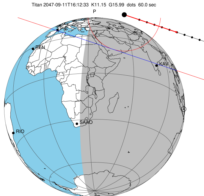
2047-09-11T16:12:33.4800 α: 17 48 52.2224 δ: -22 30 48.411 C/A 0.968" PA 18.51 deg v_sky + 9.35 km/s D 09.84 AU Credit: Styled after SORA/Lucky Star
