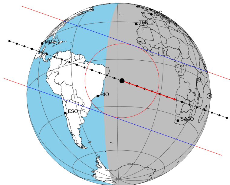
2047-09-11T20:24:33.6000 α: 17 48 53.5821 δ: -22 30 54.024 C/A 0.137" PA 19.52 deg v_sky + 9.20 km/s D 09.84 AU
