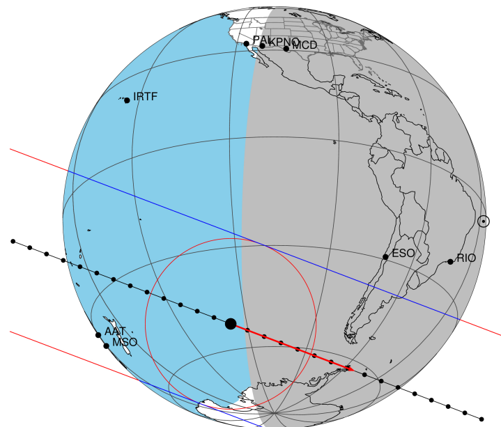
2047-09-12T01:38:38.3400 α: 17 48 55.2246 δ: -22 31 01.720 C/A 0.484" PA 200.81 deg v_sky + 8.99 km/s D 09.85 AU Credit: Styled after SORA/Lucky Star
