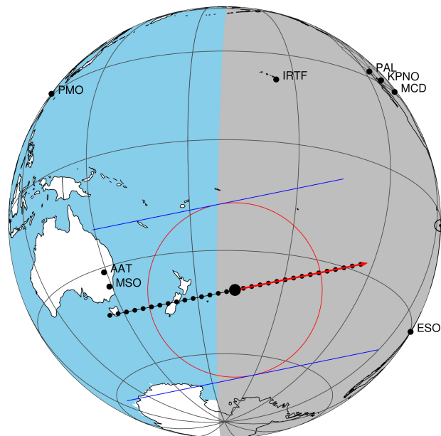
2047-09-19T05:20:34.6500 α: 17 49 20.0442 δ: -22 33 51.639 C/A 0.279" PA 168.50 deg v_sky + 4.20 km/s D 09.95 AU
